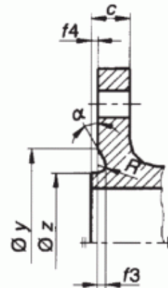
Type H: O-ring groove
